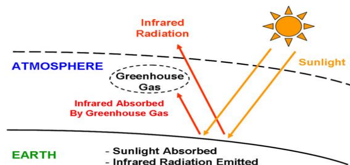
Figure 2. Greenhouse effect
